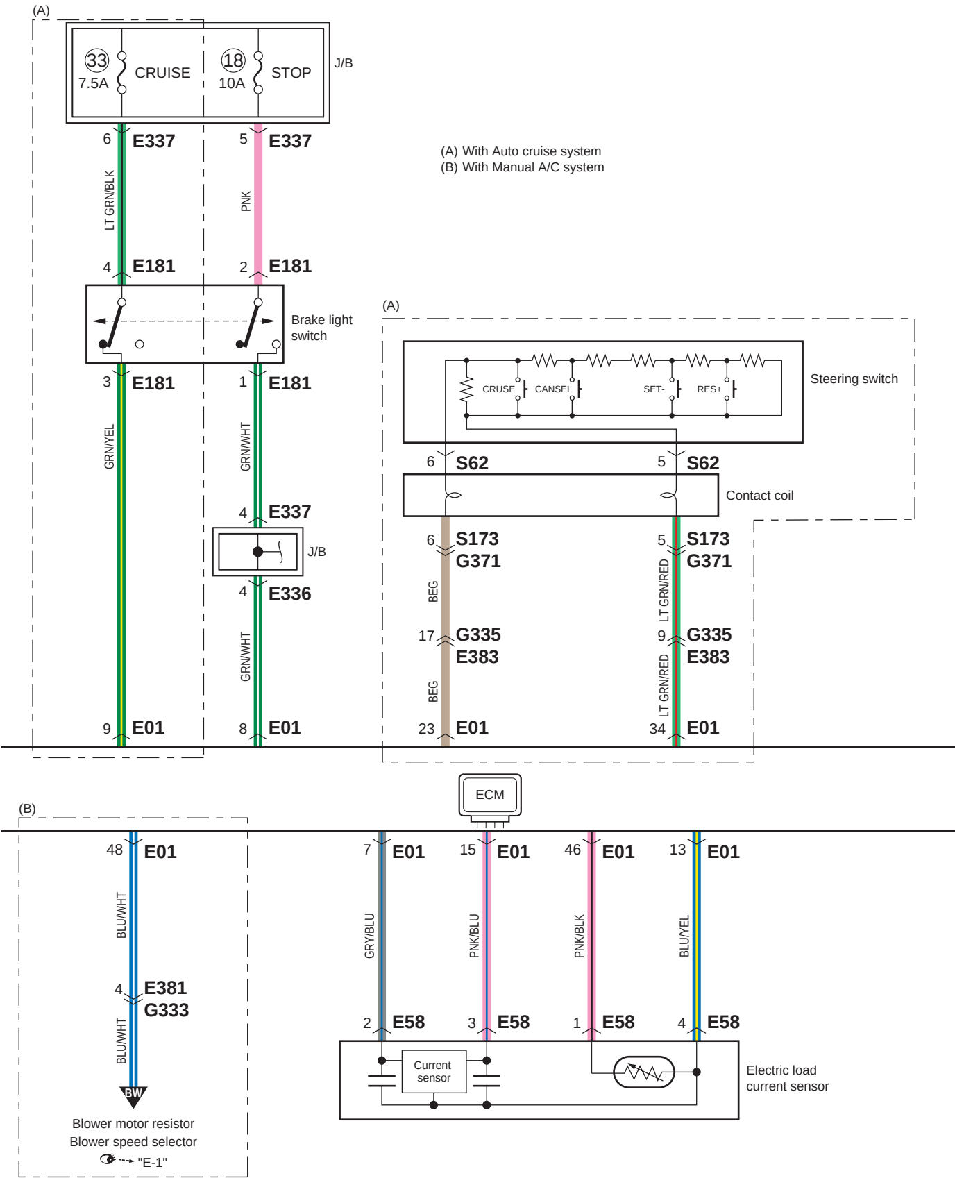
A-5-1 Engine and A/C Control System Circuit Diagram (Petrol Model)
