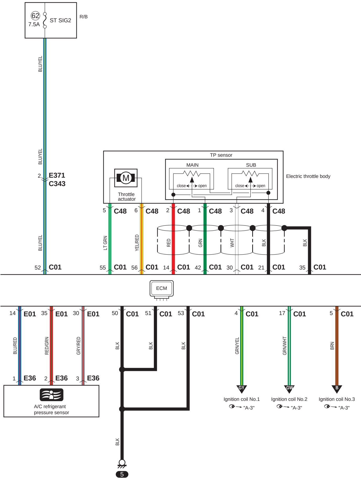
A-5-1 Engine and A/C Control System Circuit Diagram (Petrol Model)
