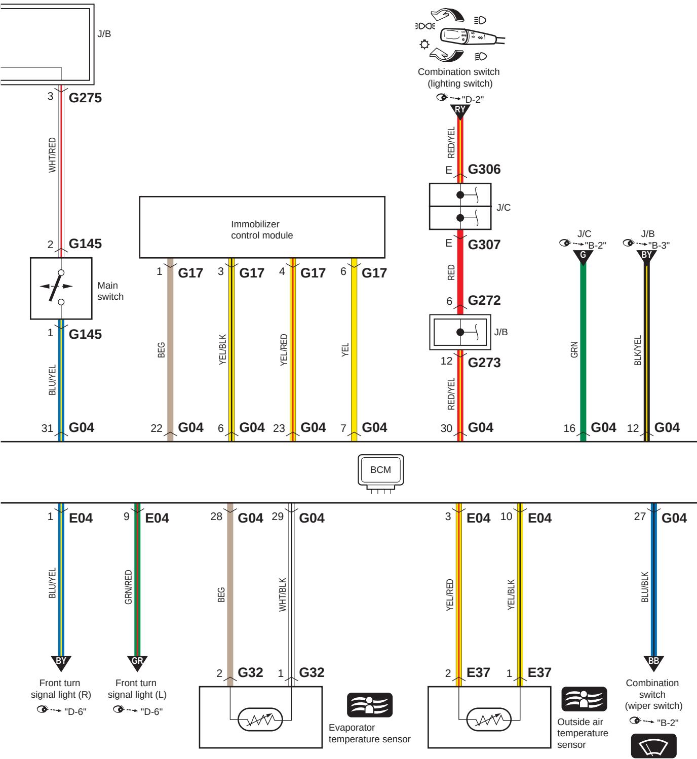
A-8-1 Body Control System Circuit Diagram (Without Engine Push Start System)
