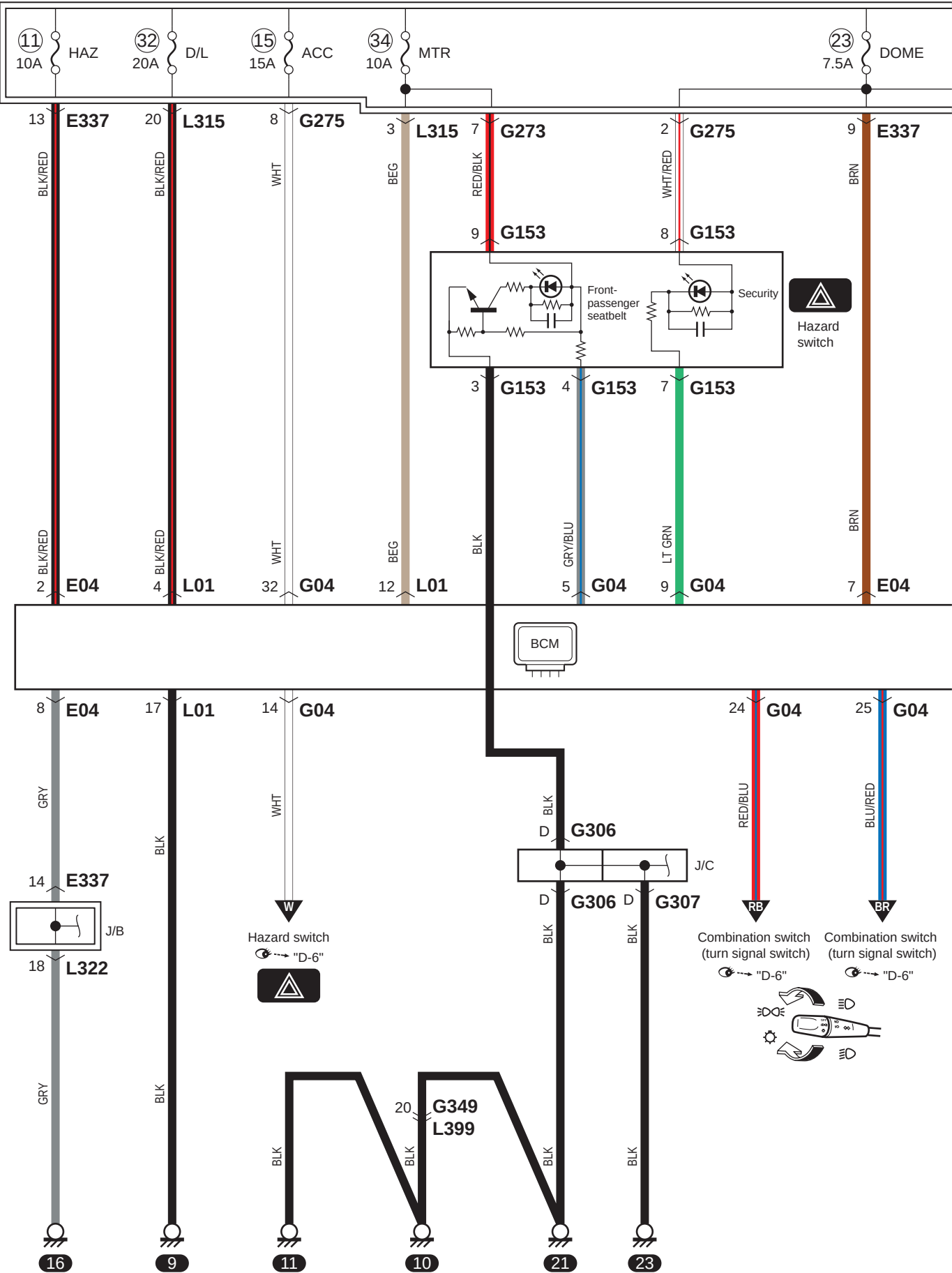
A-8-1 Body Control System Circuit Diagram (Without Engine Push Start System)
