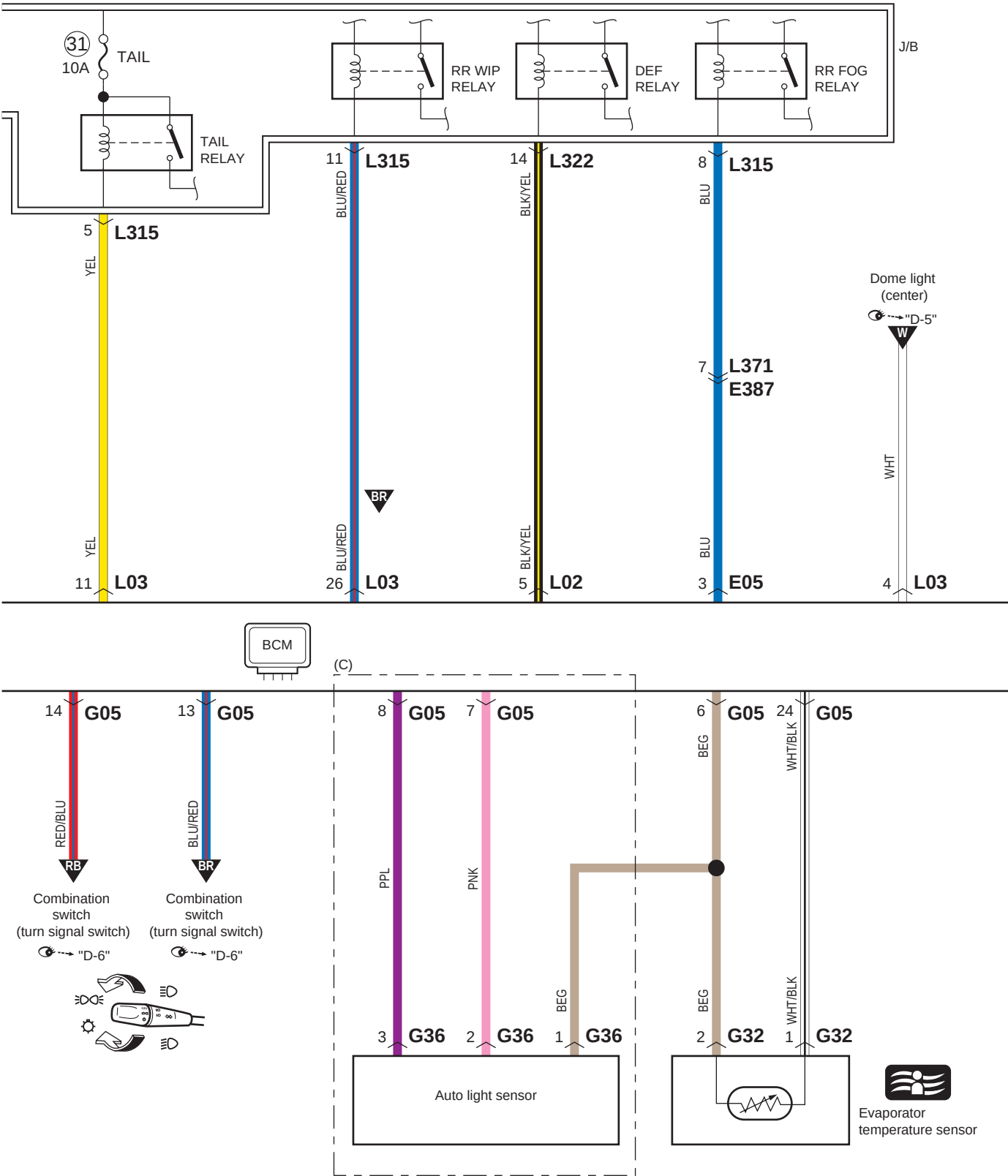
A-8-2 Body Control System Circuit Diagram (With Engine Push Start System)
