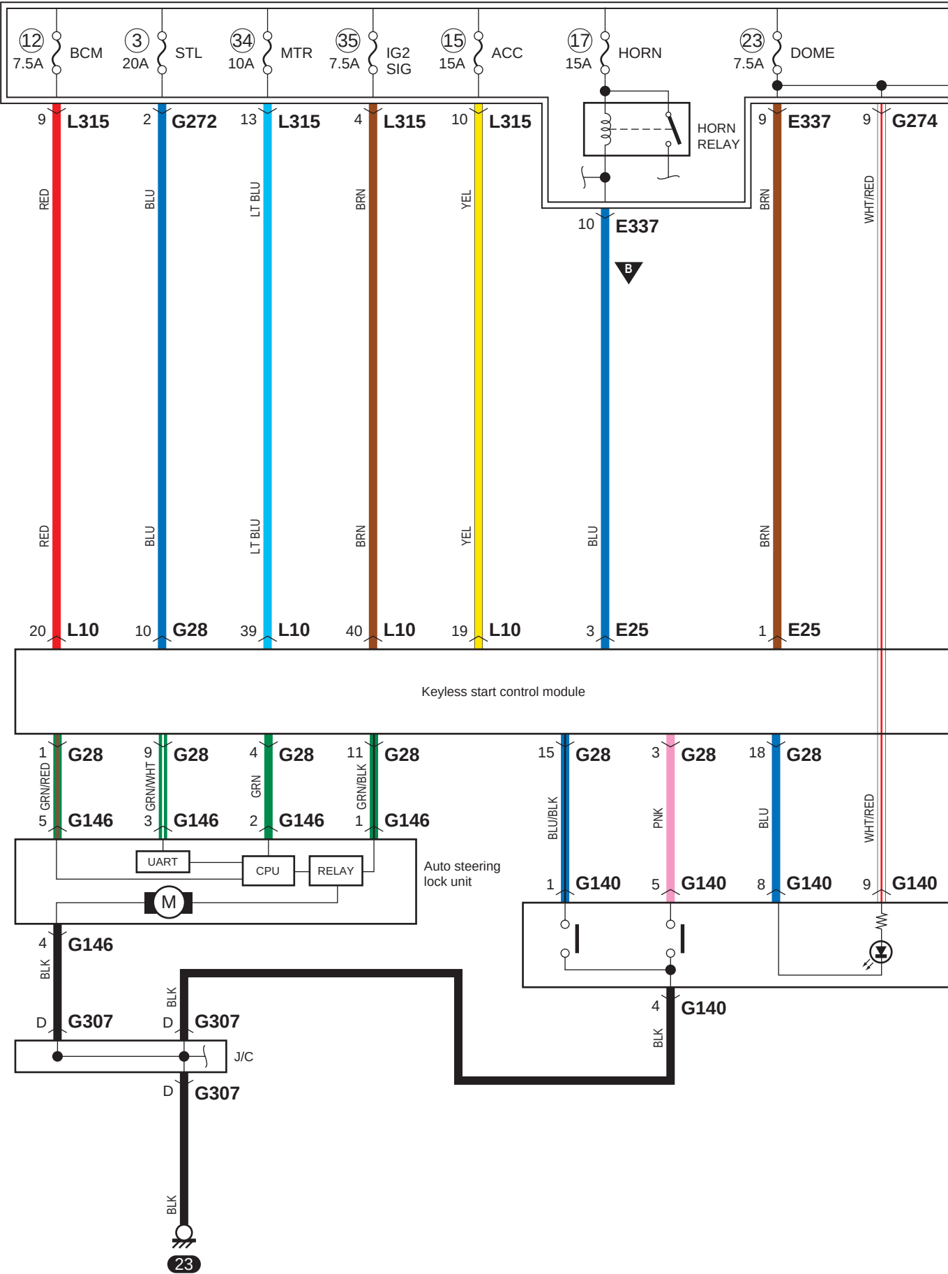
A-10 Keyless-security Control System Circuit Diagram (With Engine Push Start System)
