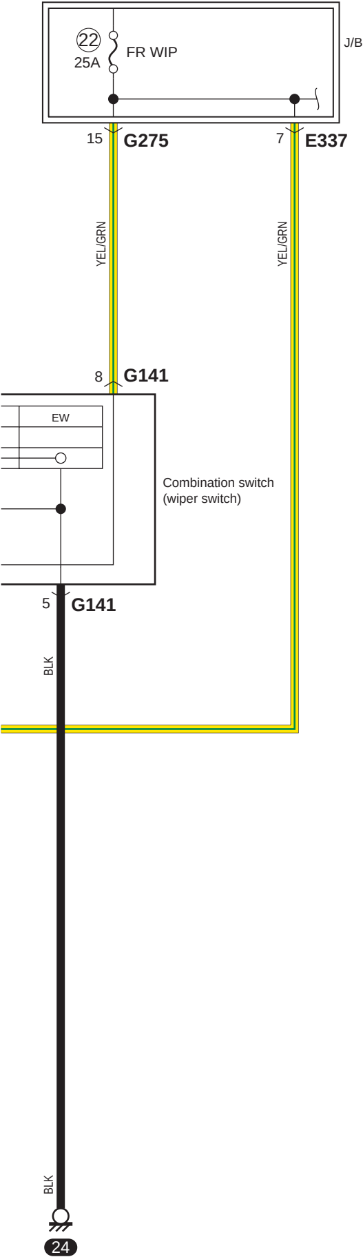
B-1 Windshield Wiper and Washer Circuit Diagram
