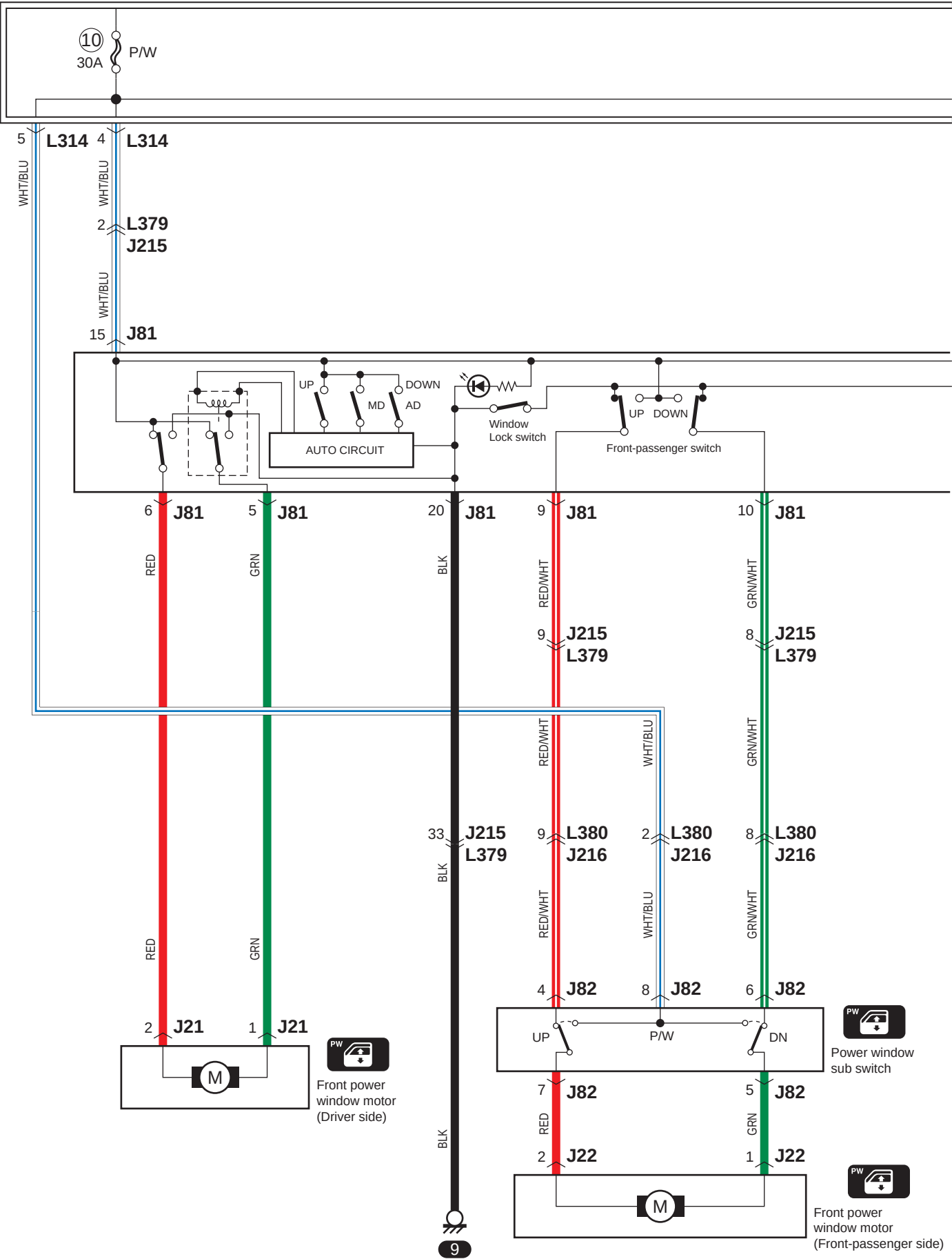
B-4 Power Window Circuit Diagram
