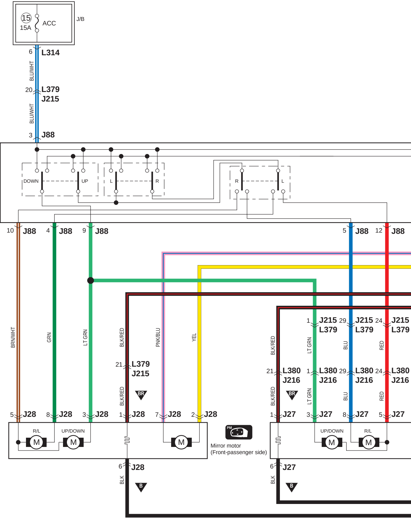
B-6-2 Power Mirror Circuit Diagram (LHD Model)
