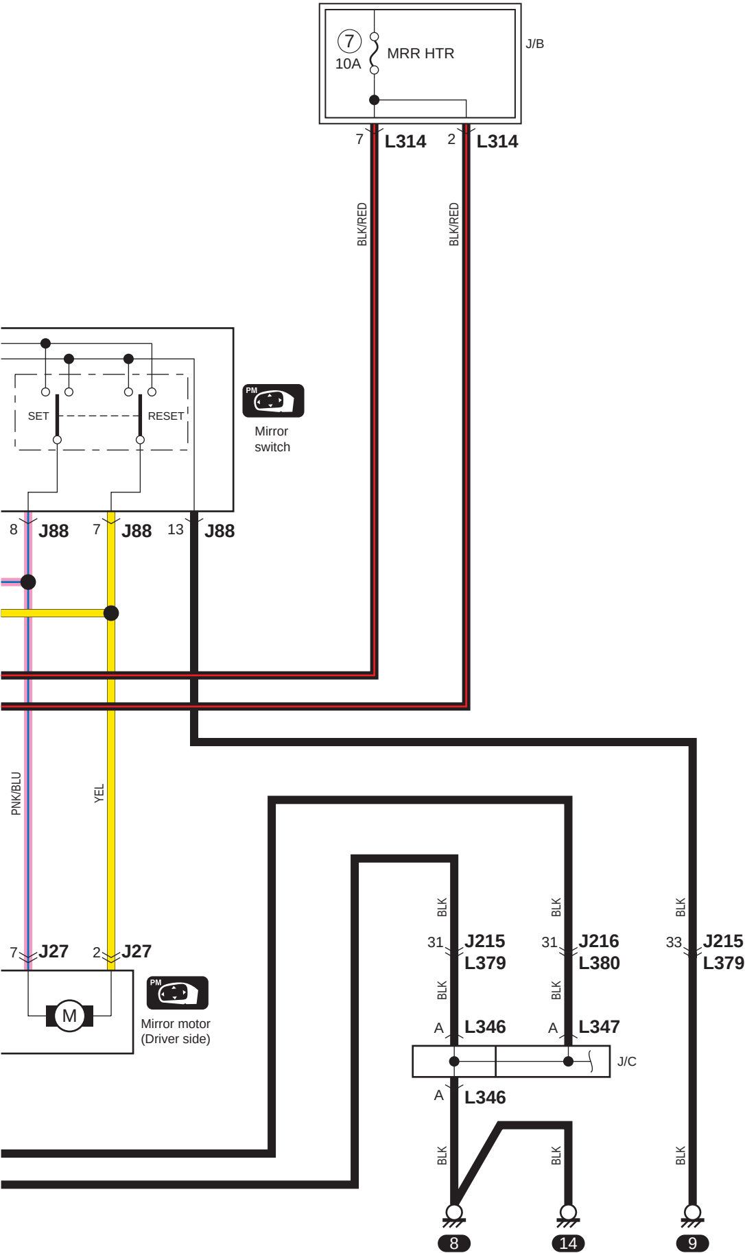
B-6-2 Power Mirror Circuit Diagram (LHD Model)
