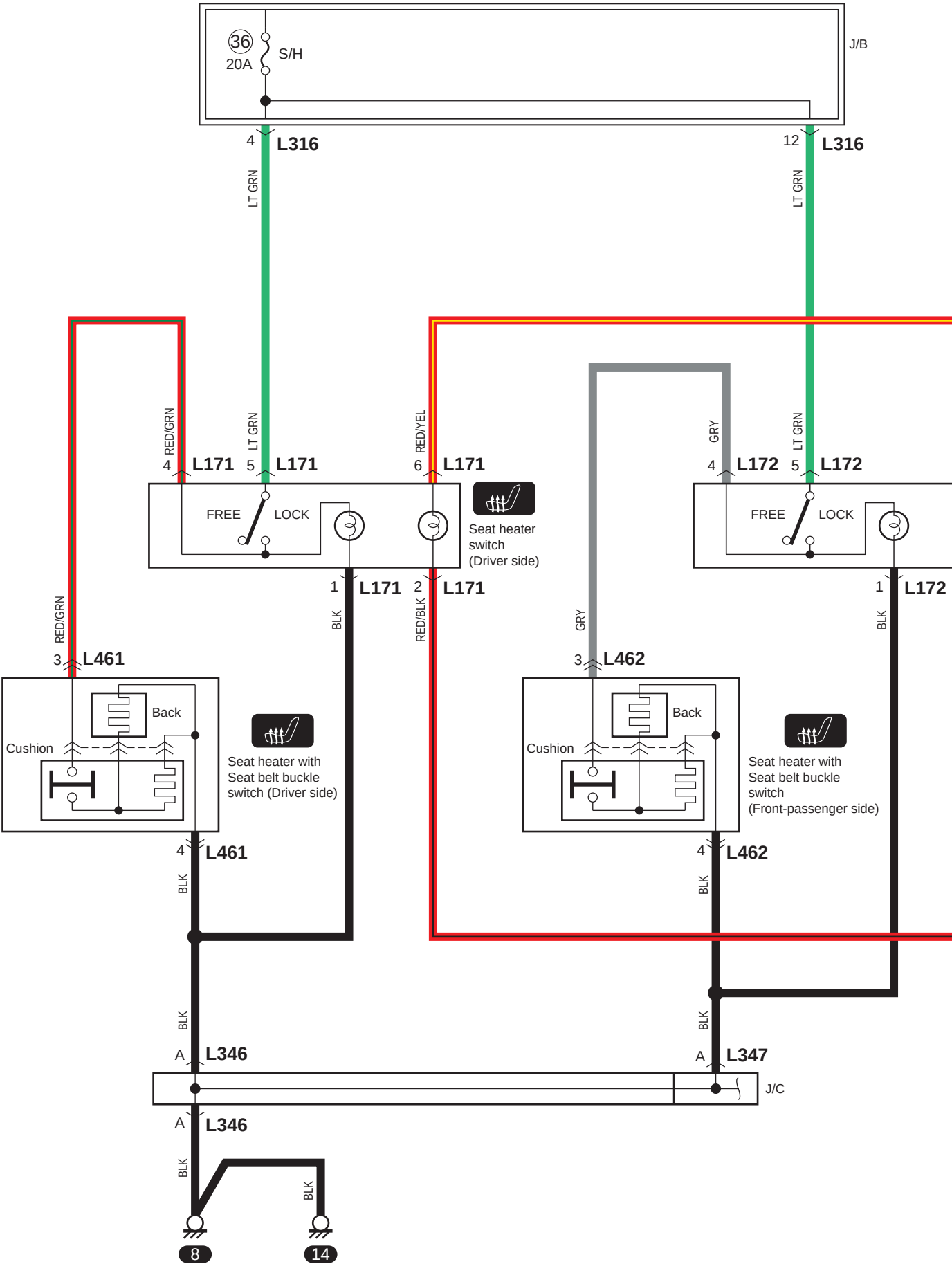
B-8 Seat Heater Circuit Diagram
