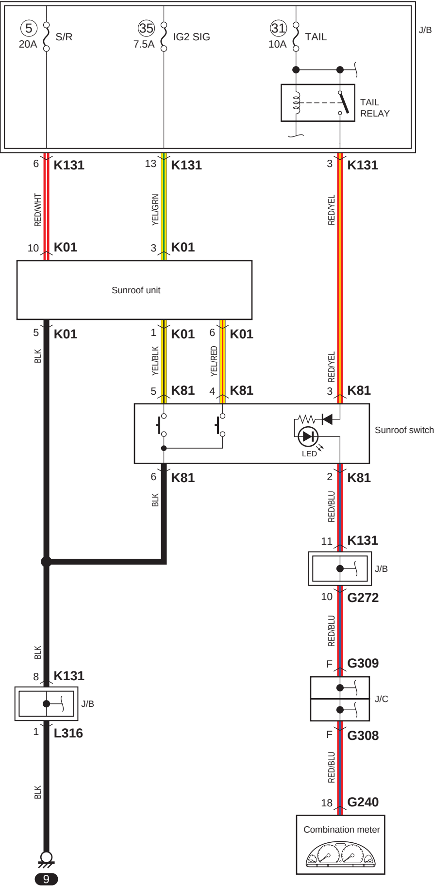
B-9 Sunroof Circuit Diagram
