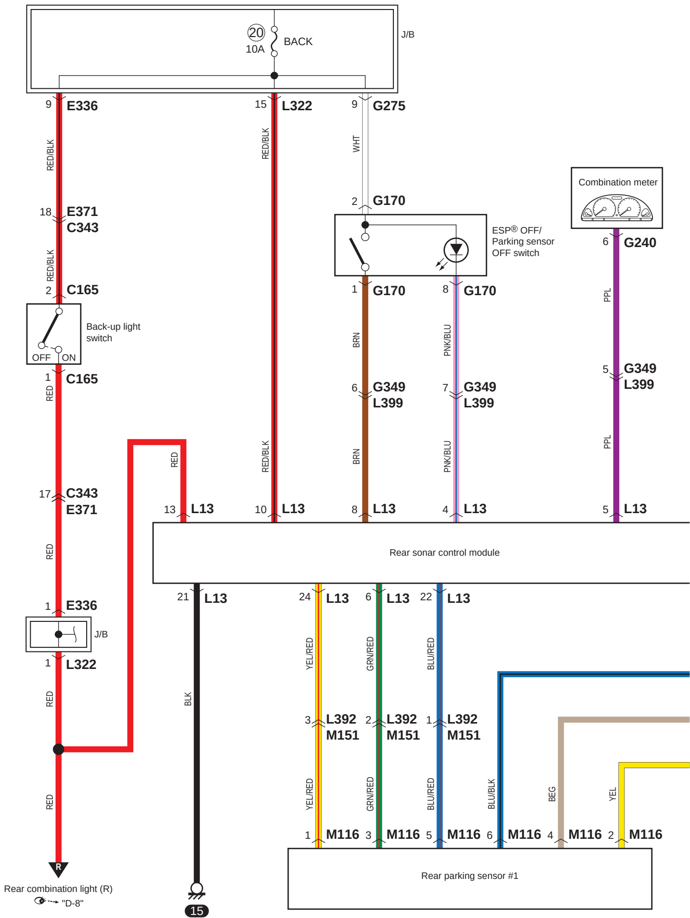
B-11 Parking Sensor System Circuit Diagram
