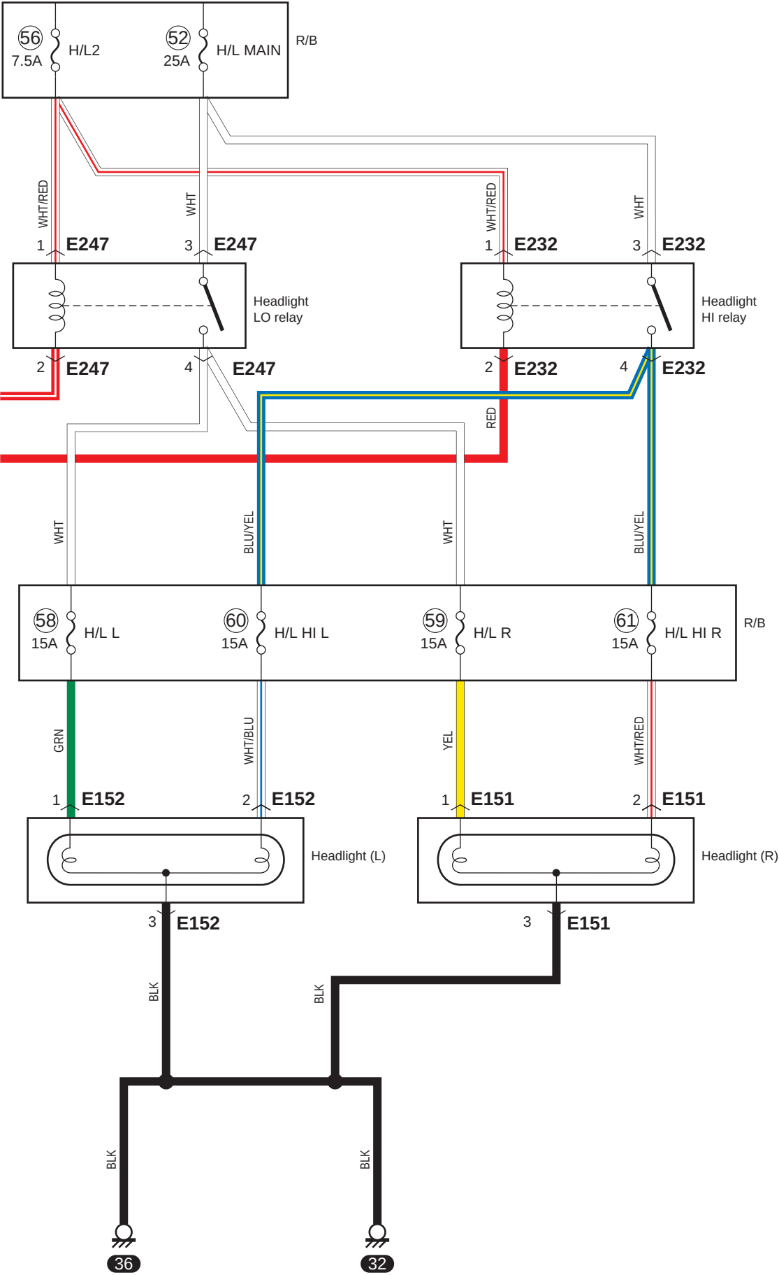
D-1-2 Headlight System Circuit Diagram (With Engine Push Start System)
