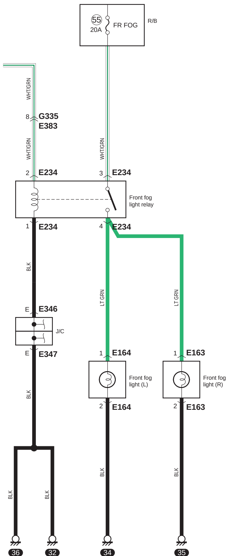
D-3-1 Front Fog Light System Circuit Diagram (Without Engine Push Start System)
