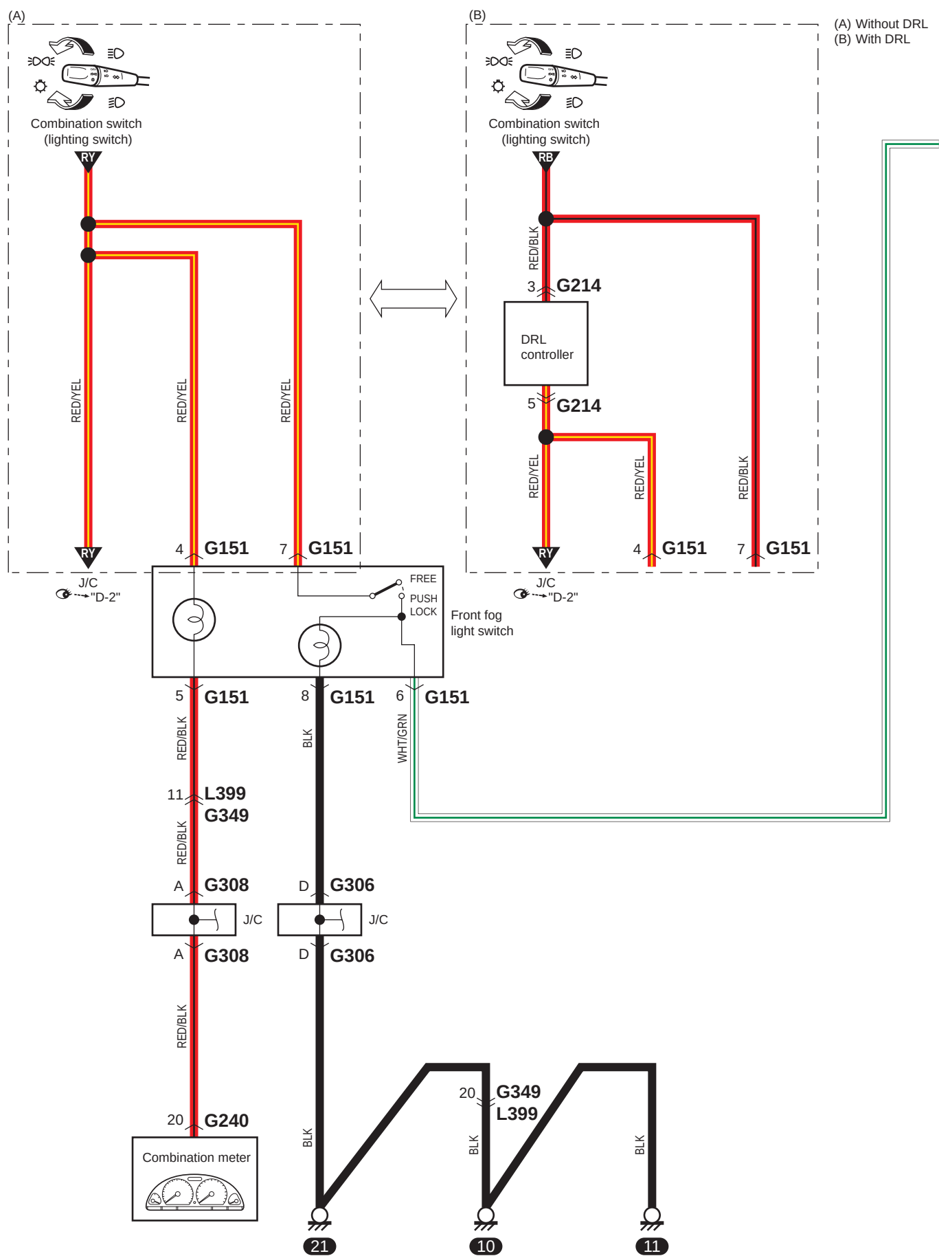
D-3-1 Front Fog Light System Circuit Diagram (Without Engine Push Start System)
