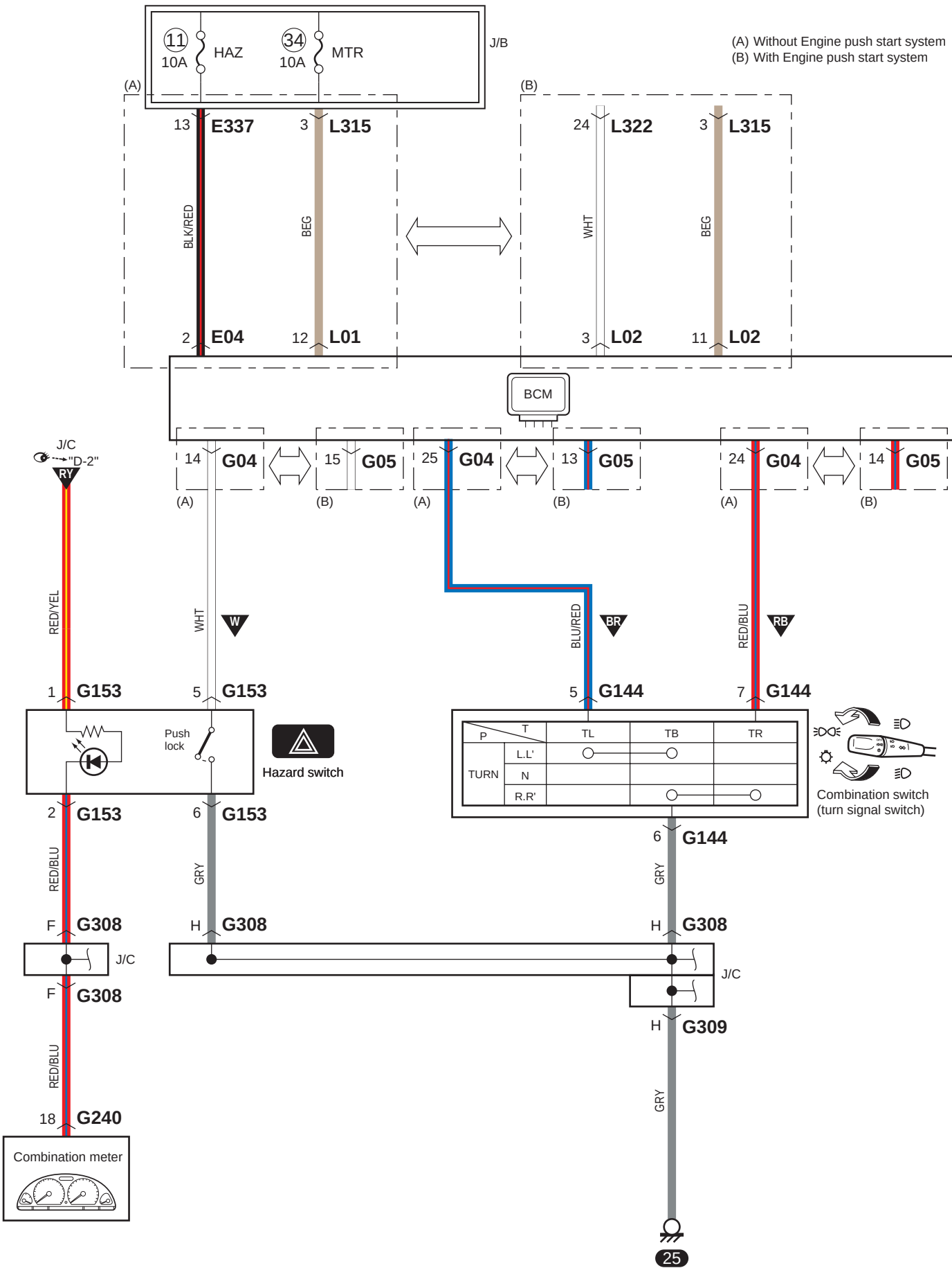
D-6 Turn Signal and Hazard Warning Light System Circuit Diagram
