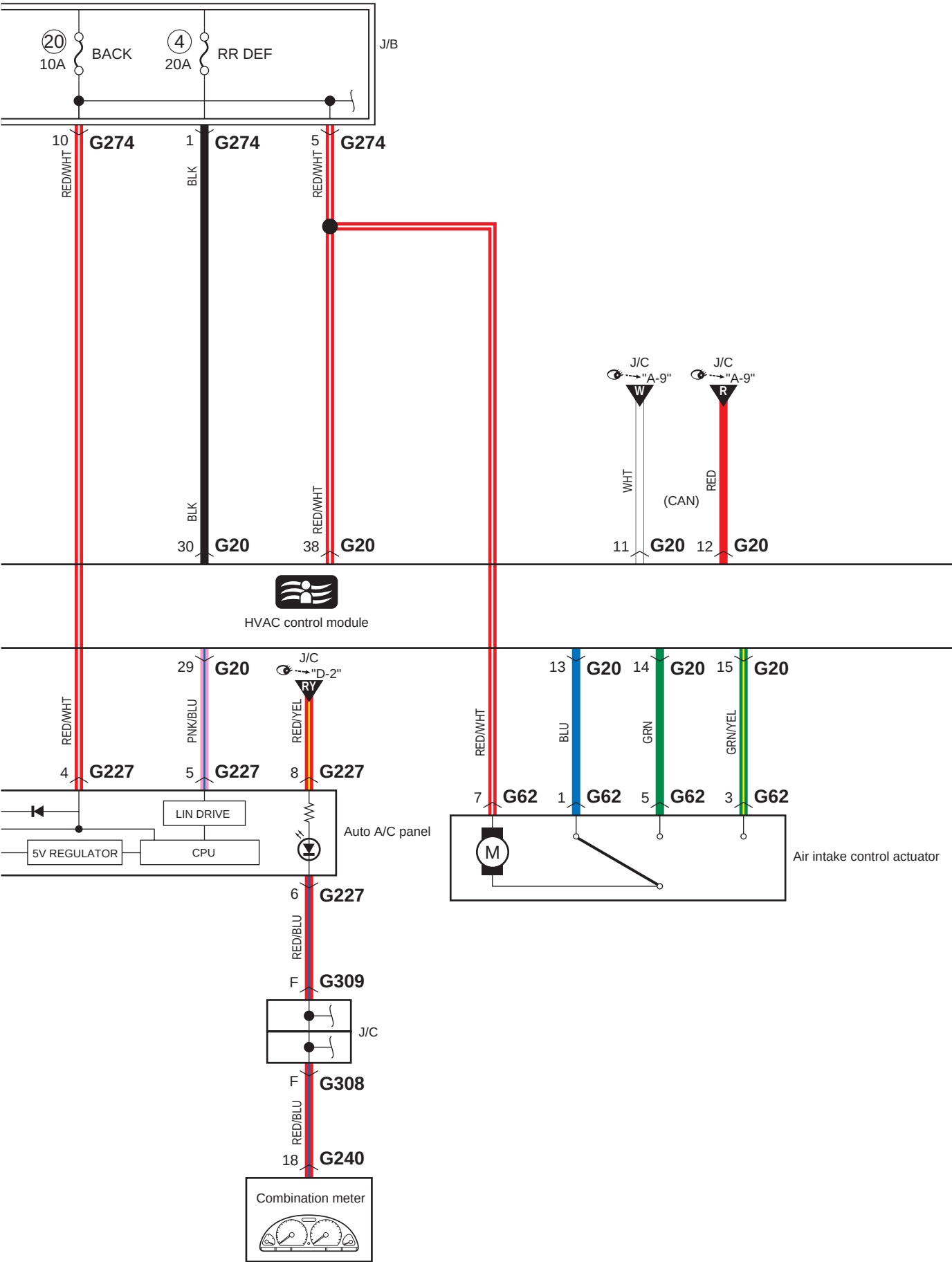
E-1-1 Auto A/C System Circuit Diagram
