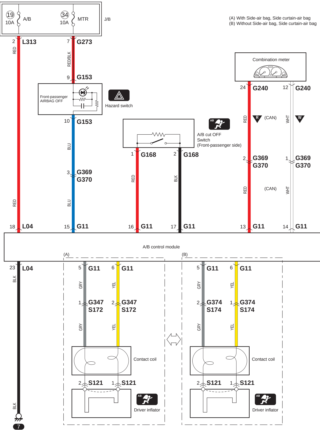
F-1 Air Bag System Circuit Diagram
