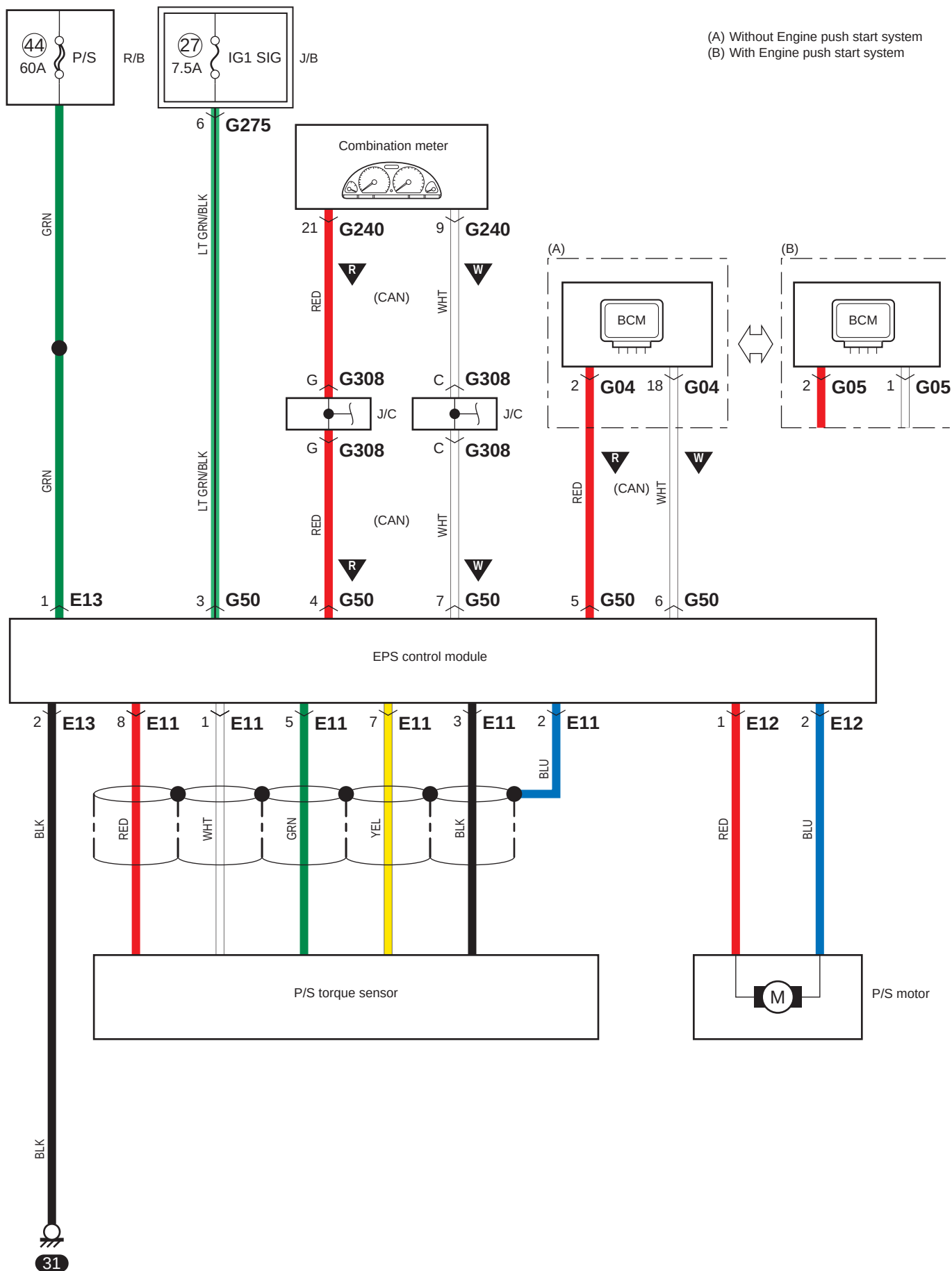
F-4 Power Steering System Circuit Diagram
