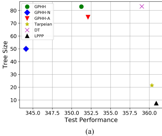
Fig. 7. Scatter map of compared approaches on representative instances. (a) Ugdb1. (b) Uval2B.
