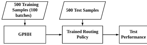
Fig. 5. Training and test phases of a GP run on a UCARP instance.
