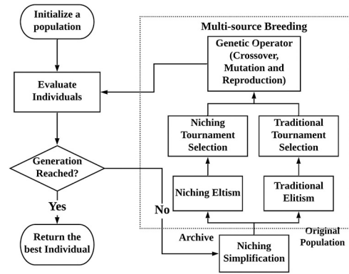
Fig. 1. Overall framework of GPHH-N.
