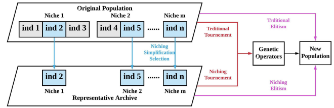
Fig. 2. Illustration of the offspring generation in GPHH-N.
