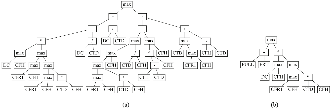
Fig. 4. Two trees with the same fitness but different tree sizes. (a) Tree A. (b) Tree B.
