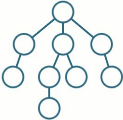
DFS
