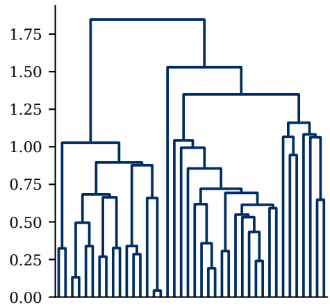
linkage single
