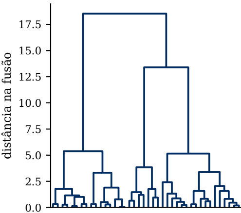
linkage ward
