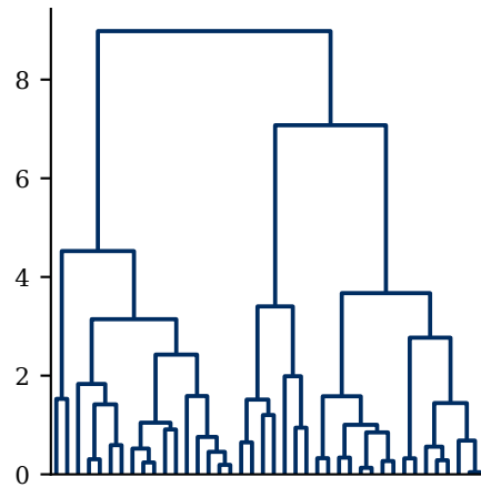
linkage complete
