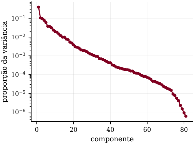
scree plot
