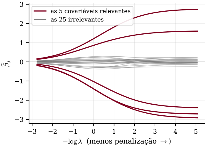
Ridge ( \ell_2 )
