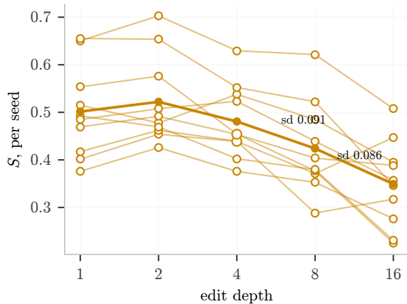
Ten seeds, still spread at depth sixteen
