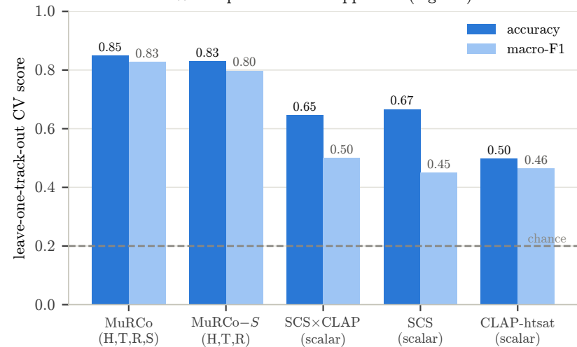
Which perturbation happened? (logistic)
