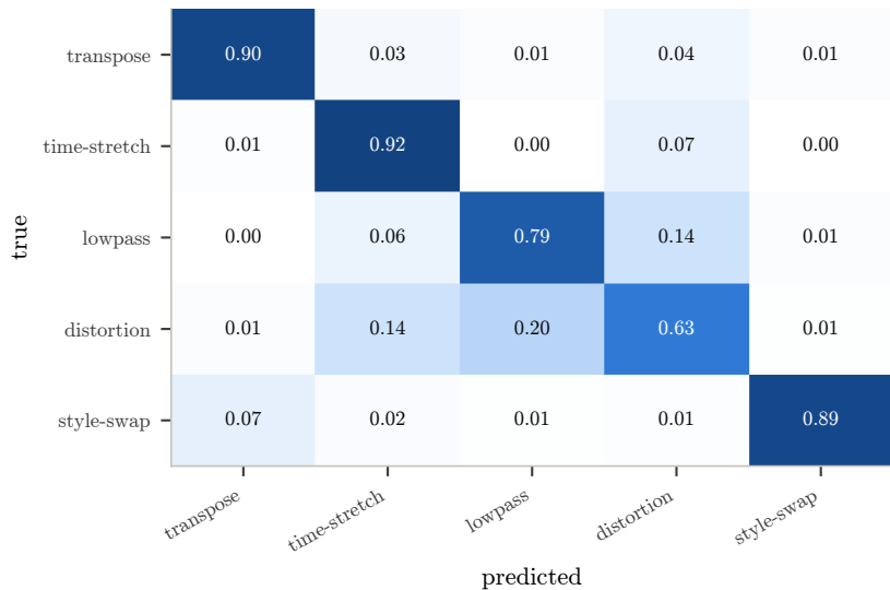
MuRCo (H,T,R,S) confusion, row-normalised
