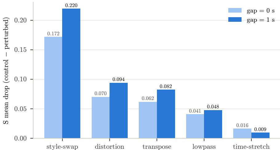
Gap ablation (M.1): the 1 s gap sharpens style-swap separation
