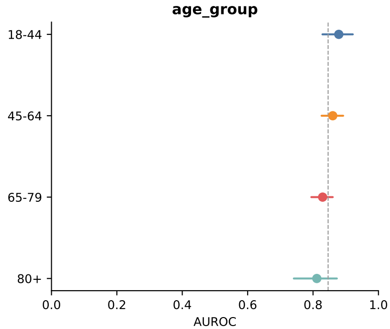
Figure 1. Subgroup AUROC with bootstrap CIs (SUPPORT2)
