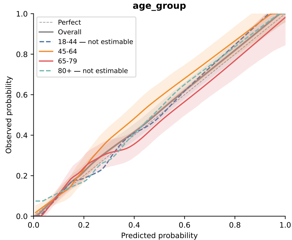
Figure 2. Subgroup calibration curves (SUPPORT2)
