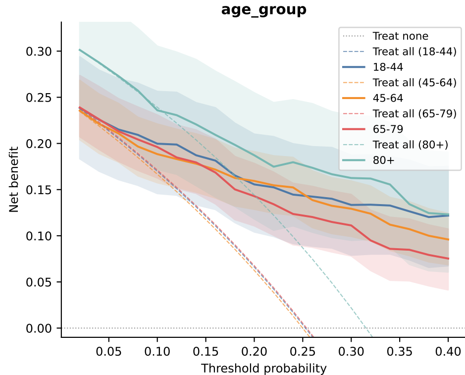
Figure 3. Subgroup decision curves (SUPPORT2)
