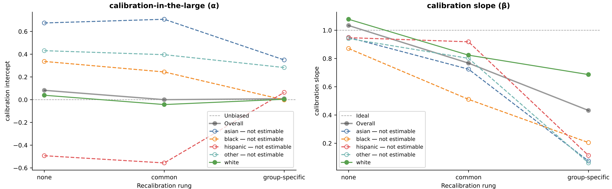
Figure 5. Recalibration ladder, race/ethnicity axis (SUPPORT2)
