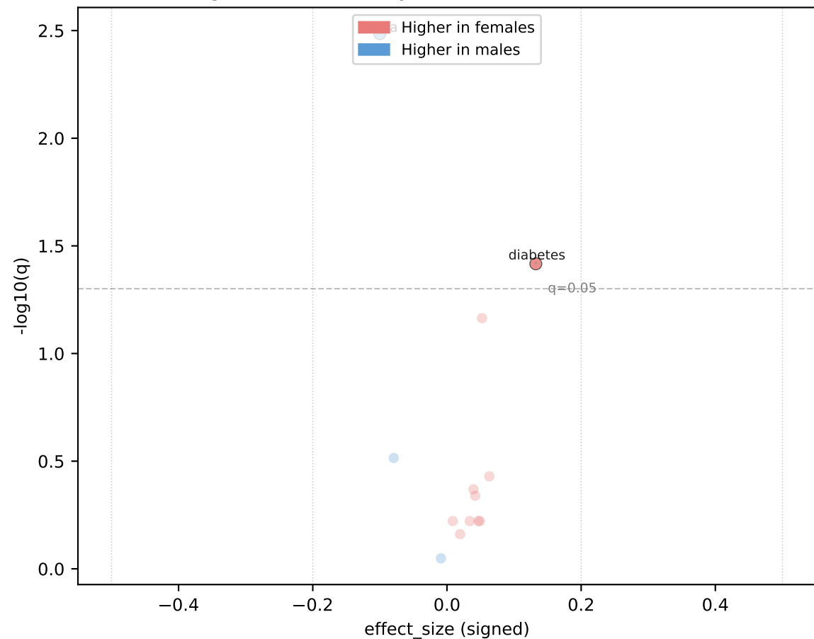
Figure 6A. Feature-by-sex effect sizes (SUPPORT2)
