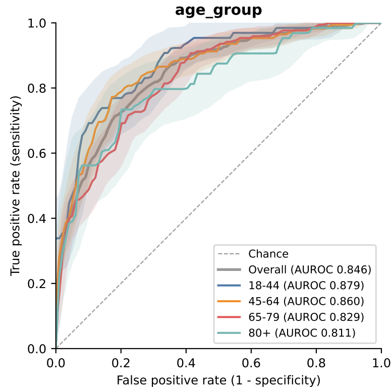
Supplementary Figure — per-subgroup ROC (SUPPORT2)
