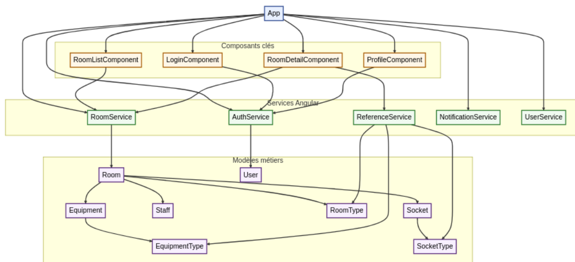
FIGURE 5.1 – Schéma d'architecture applicative - Angular
