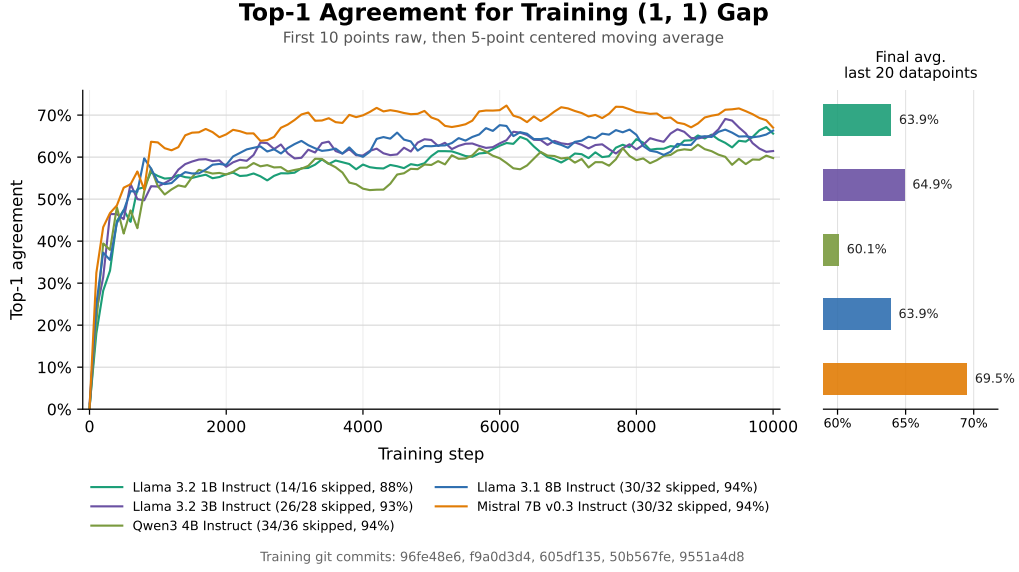
Figure 17: Top-1 agreement between drafter and verifier during training for the (1,1) gap setting. Curves show the first 10 points raw, followed by a 5-point centered moving average. The right panel reports the final average over the last 20 datapoints.
