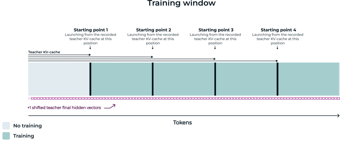
Figure 5: How a training window is structured. It is a window of context_len tokens divided into num_draft_sections sections. The vertical splitting lines indicate starting points where the student continues from how the teacher’s KV-cache was at that position. At each position it is getting the teachers t - 1 final hidden token, this is the shifted pink array, and the t position last layer hidden vector before the gap.
