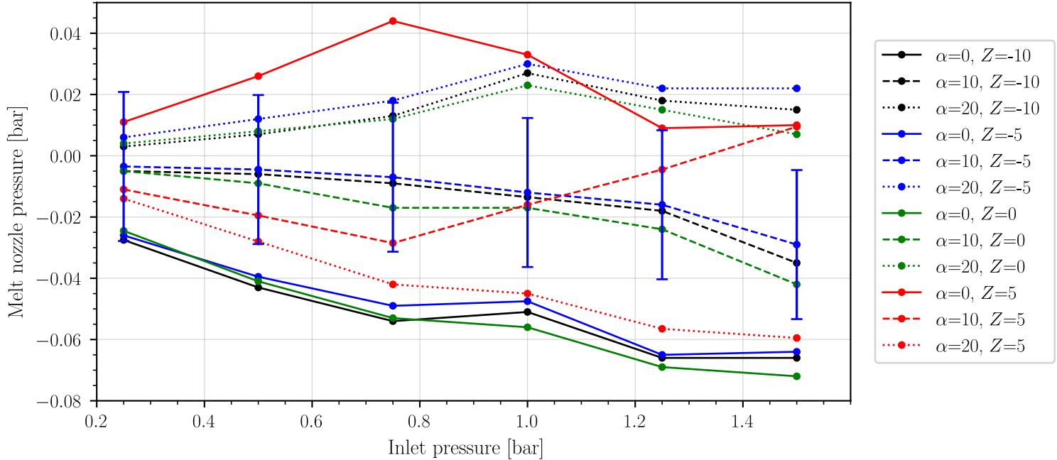
Pressure in the melt nozzle as a function of inlet pressure, varying apex angles ( \alpha ) and melt nozzle heights ( Z ) P!_Alpha!_omega_0_Z!_DJ_1.5_RJ_6_AnSl_Reg
