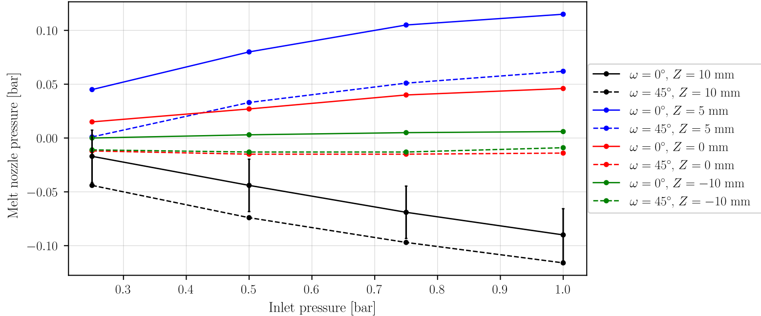
Pressure in the melt nozzle as a function of inlet pressure, varying swirl angle ( \omega ) and vertical shift ( Z ) P_!_Alpha_0_omega_!_Z_!_DJ_1.5_RJ_6_AnSl_Reg
