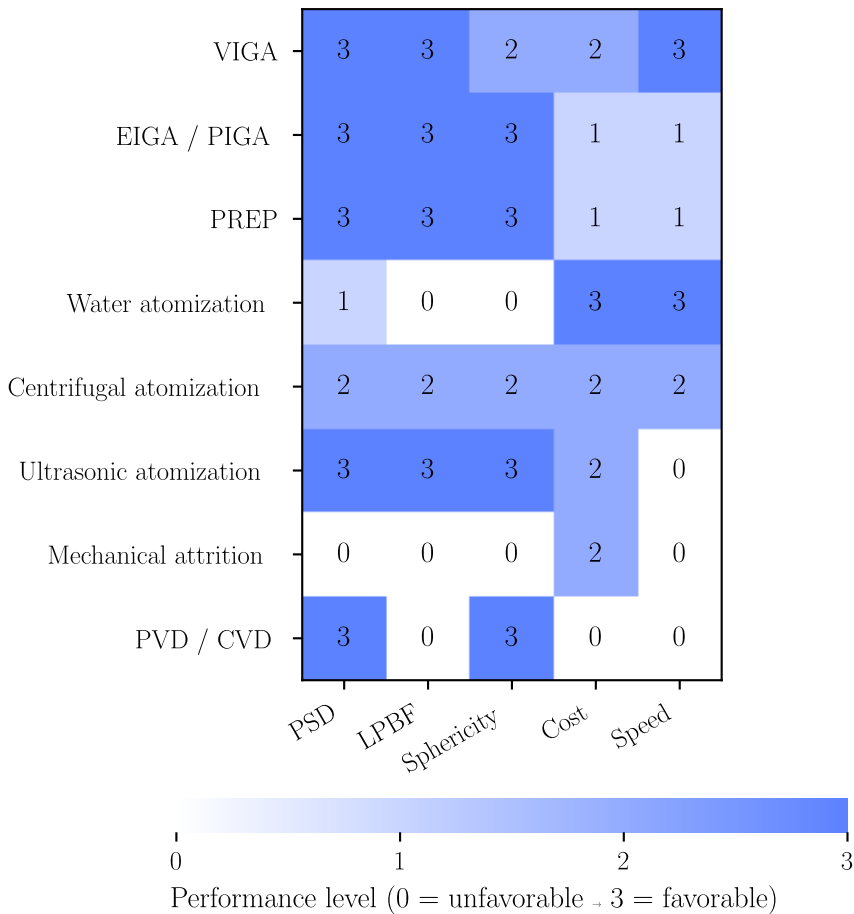
Comparative Assessment of Powder Production Routes
