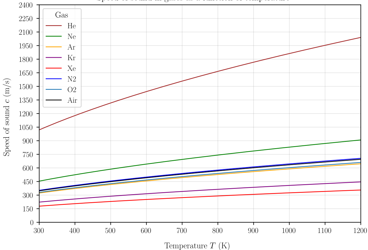
Speed of sound in gases as a function of temperature
