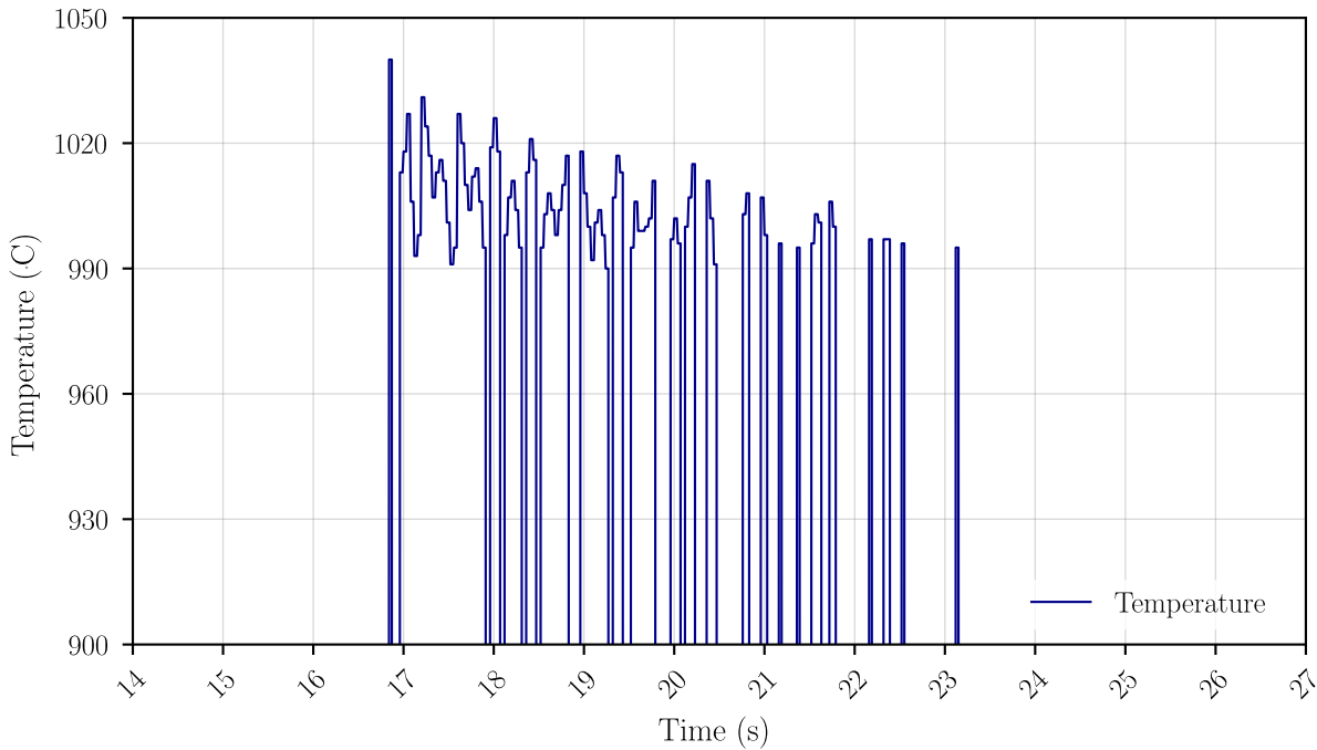
Furnace Temperature
