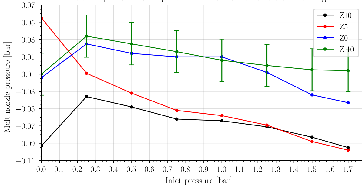
Pressure in the melt nozzle as a function of stage 1 inlet pressure ( P_1 ), keeping stage 2 at 0.72 bar ( P_2 ), varying gas nozzles vertical shift ( Z ) P_!_0.72_Alpha_3_14_Omega_45_45_Z!_DJ_1.5_1.5_RJ_6_7.5_AnSl_Reg
