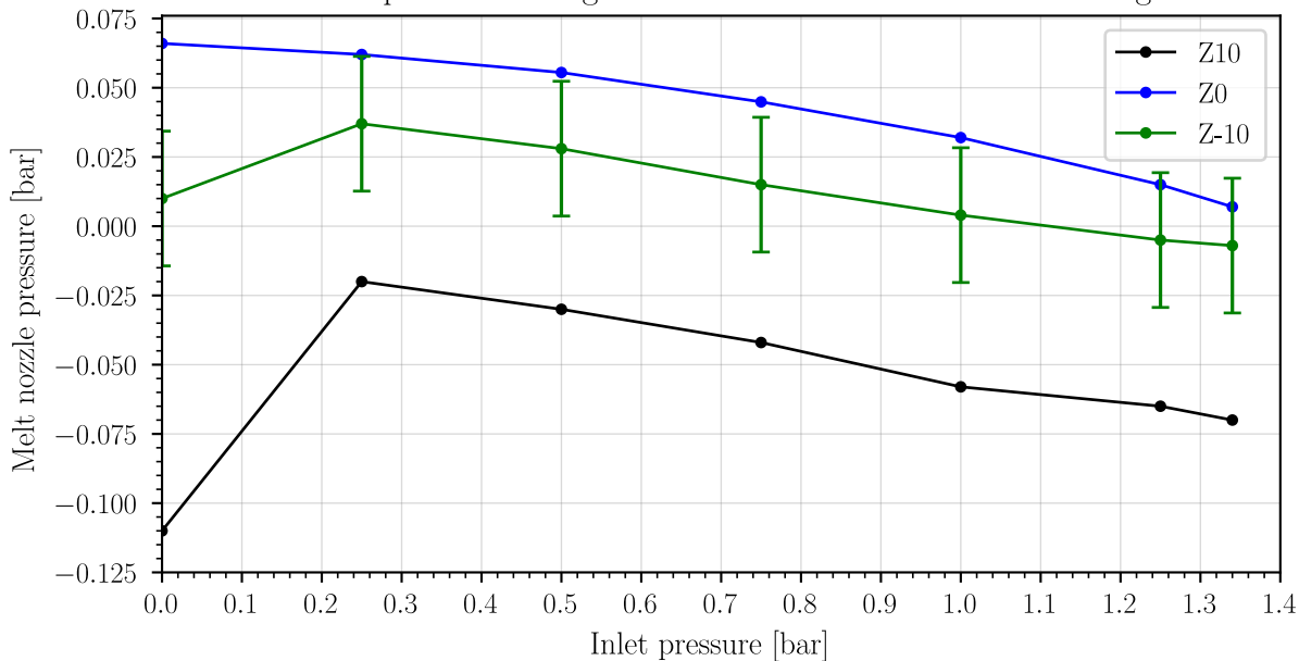
Pressure in the melt nozzle as a function of stage 1 inlet pressure ( P_1 ), keeping stage 2 at 1.07 bar ( P_2 ), varying gas nozzles vertical shift ( Z ) P!_1.07_Alpha_3.14_Omega_0.0_Z!_DJ_1.5_1.5_RJ_6.7.5_AnSl_Reg
