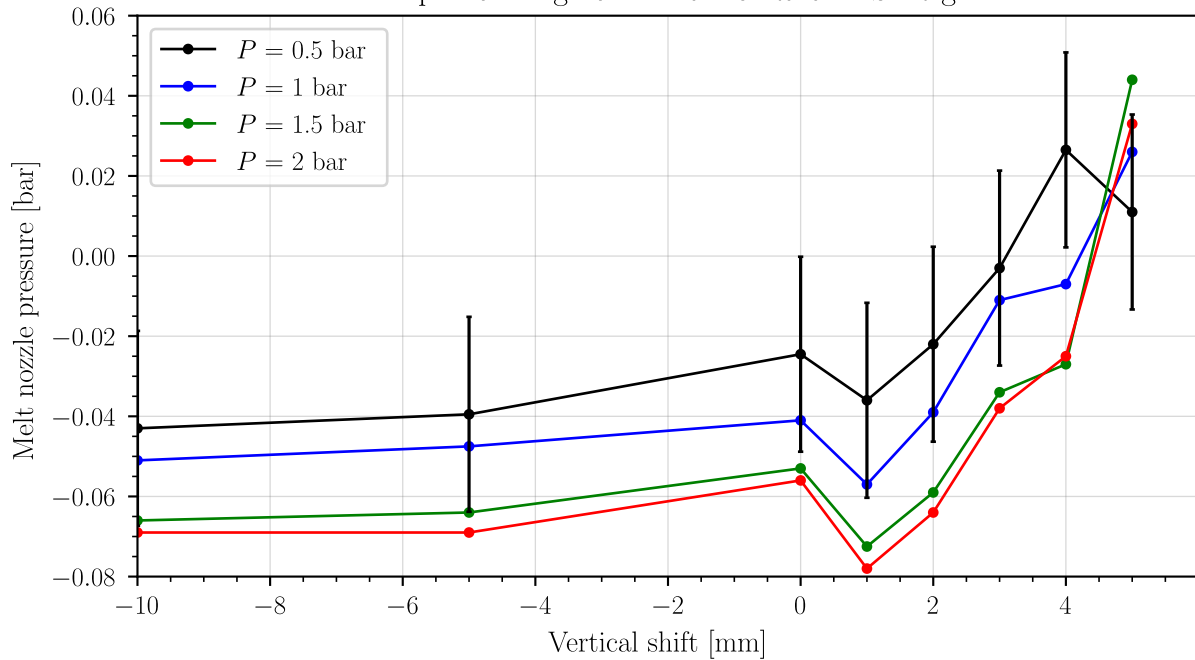
Pressure in the melt nozzle as a function of gas nozzle vertical shift ( Z ), varying inlet pressure ( P ) P_!_Alpha_0_omega_0_Z_!_DJ_1.5_RJ_6_AnSl_Reg
