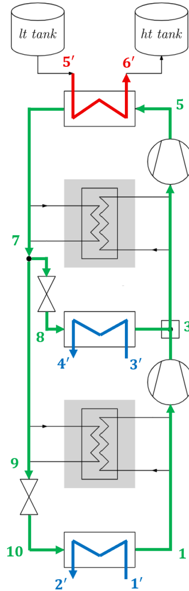
Figure 3: Schematic of the Dual-Evaporator Subcritical Heat Pump cycle (SC2)
