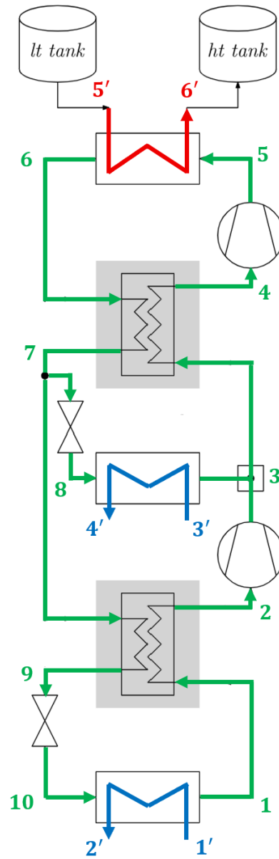
Figure 4: Schematic of the Dual-Evaporator Subcritical Heat Pump cycle with Recuperator (SC2R)
