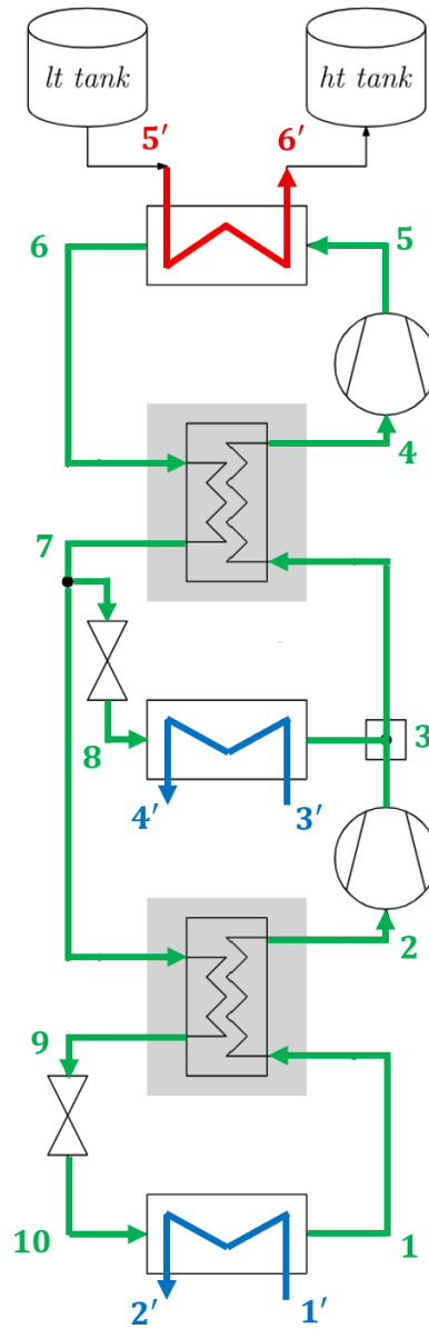
Figure 8: Schematic of the Dual-Evaporator Transcritical Heat Pump cycle with Recuperator (TC2R)
