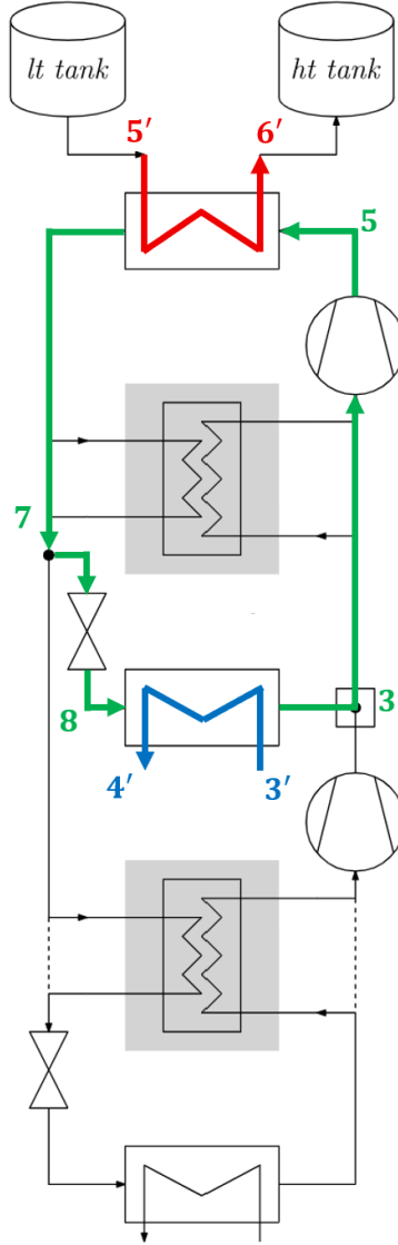
Figure 5: Schematic of the One Evaporator Transcritical Heat Pump cycle (TC1)
