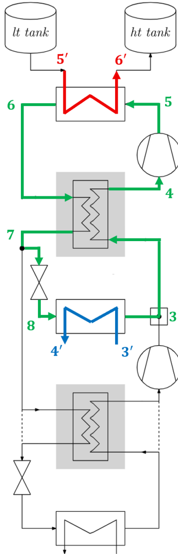
Figure 6: Schematic of the One Evaporator Transcritical Heat Pump cycle with Recuperator (TC1R)
