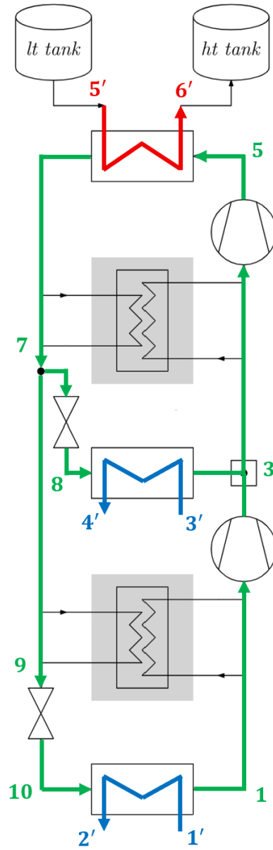
Figure 7: Schematic of the Dual-Evaporator Transcritical Heat Pump cycle (TC2)
