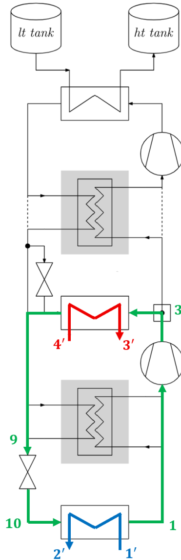
Figure 1: Schematic of the One Evaporator Subcritical Heat Pump cycle (SC1)
