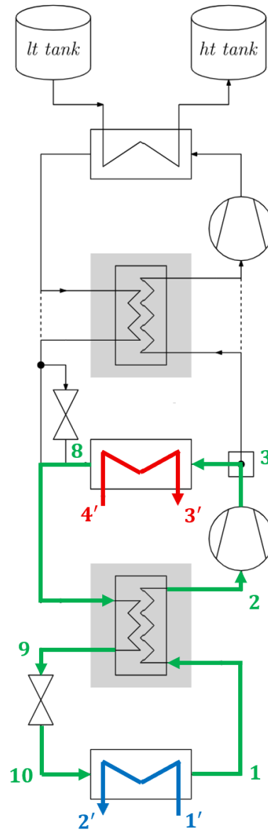
Figure 2: Schematic of the One Evaporator Subcritical Heat Pump cycle with Recuperator (SC1R)
