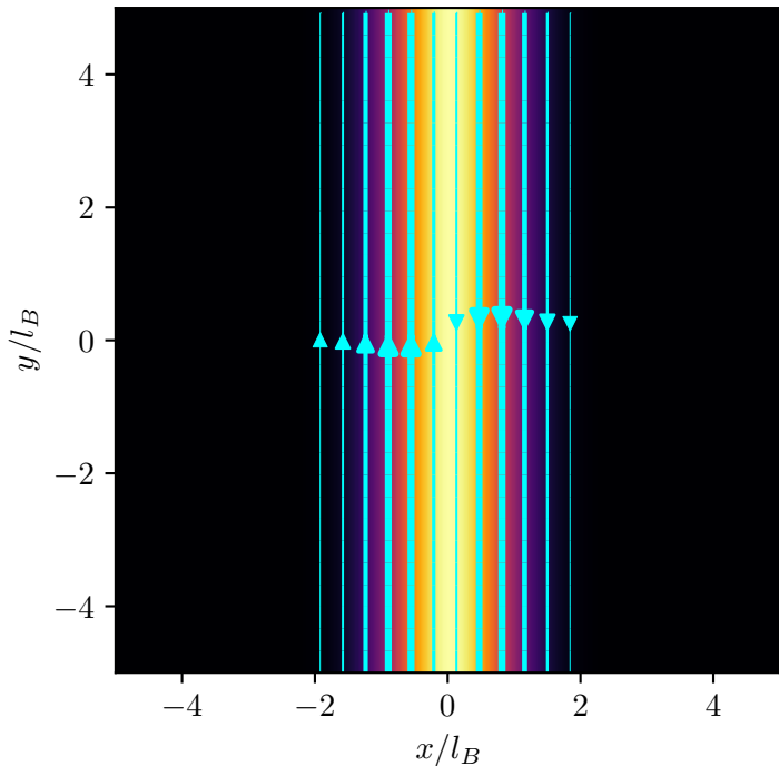
Orbital Current \vec{J}_{orb}
