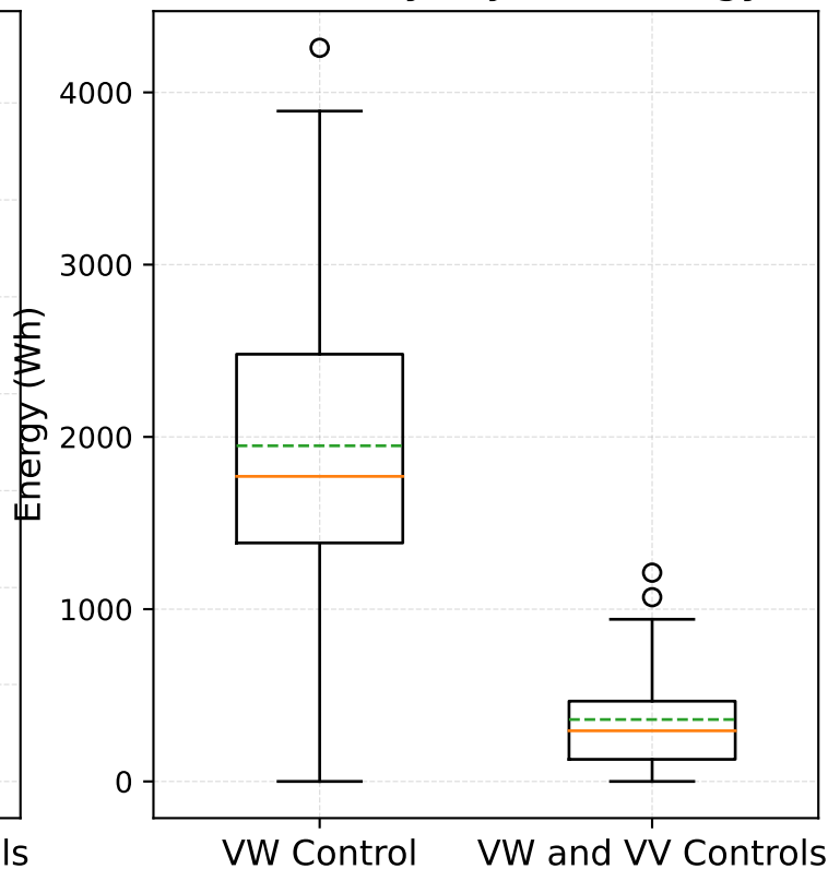
(B) Battery Adjusted Energy
