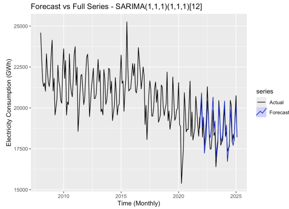
(a) Modelo SARIMA(1,1,1)(1,1,1)[12].
