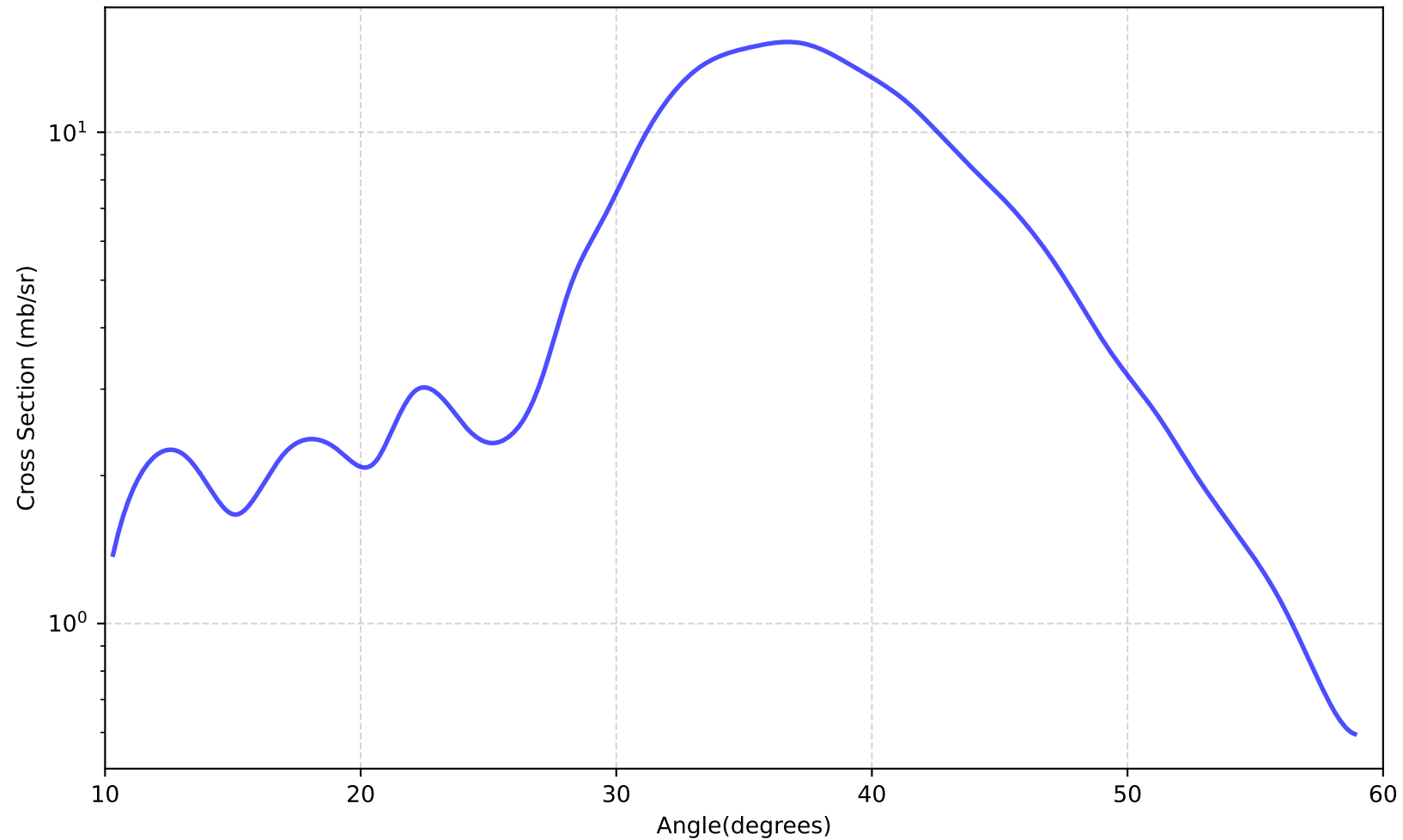
^{90}\text{Zr}(^{12}\text{C}, ^{13}\text{N})^{89}\text{Y}
