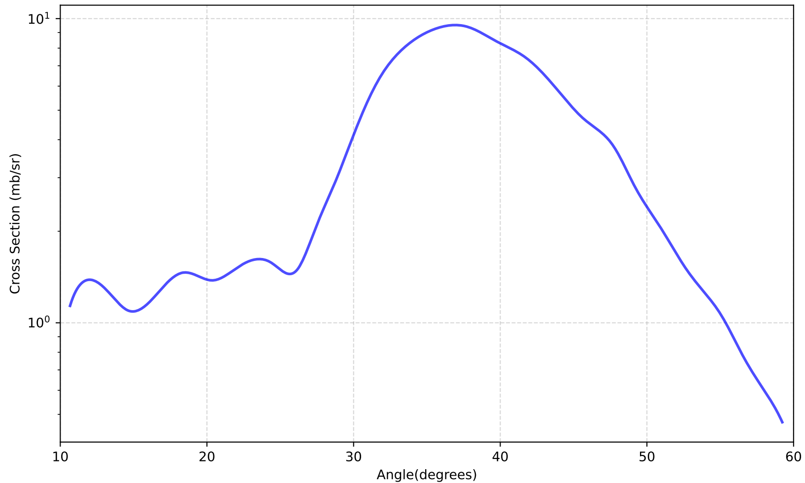
^{90}\text{Zr}(^{12}\text{C}, ^{11}\text{B})^{91}\text{Nb}
