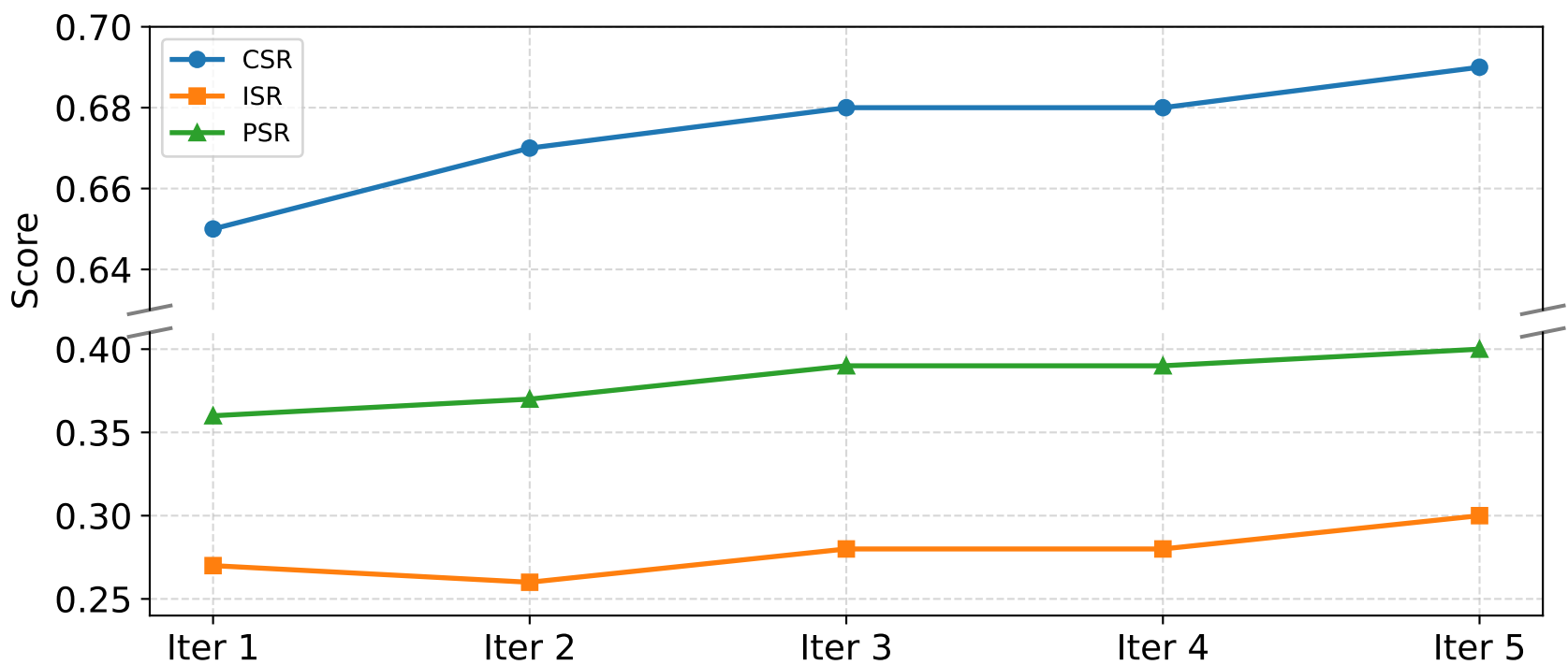
CFBench Performance
