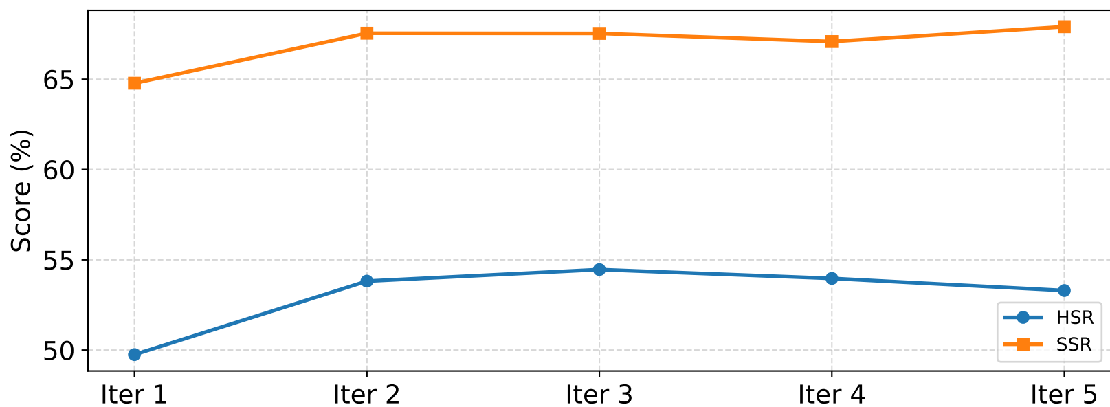
FollowBench Performance
