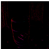
FireNet
