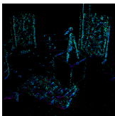
Leaky-FireFlowNet
