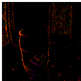
LIF-FireNet
