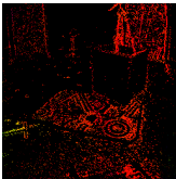
LIF-EV-FlowNet
