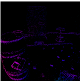
EV-FlowNet
