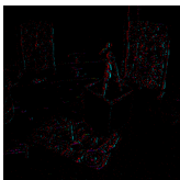
FireFlowNet
