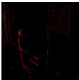
Leaky-FireNet
