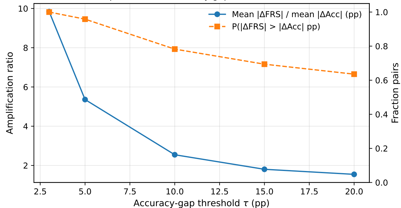
C: FRS amplification vs accuracy gap threshold (downstream)
