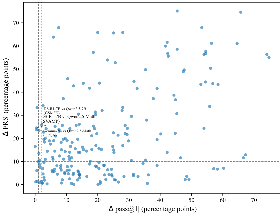
Similar pass@1 gaps can mask large FRS gaps
